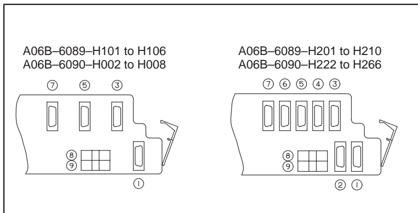
(1) Connector location
